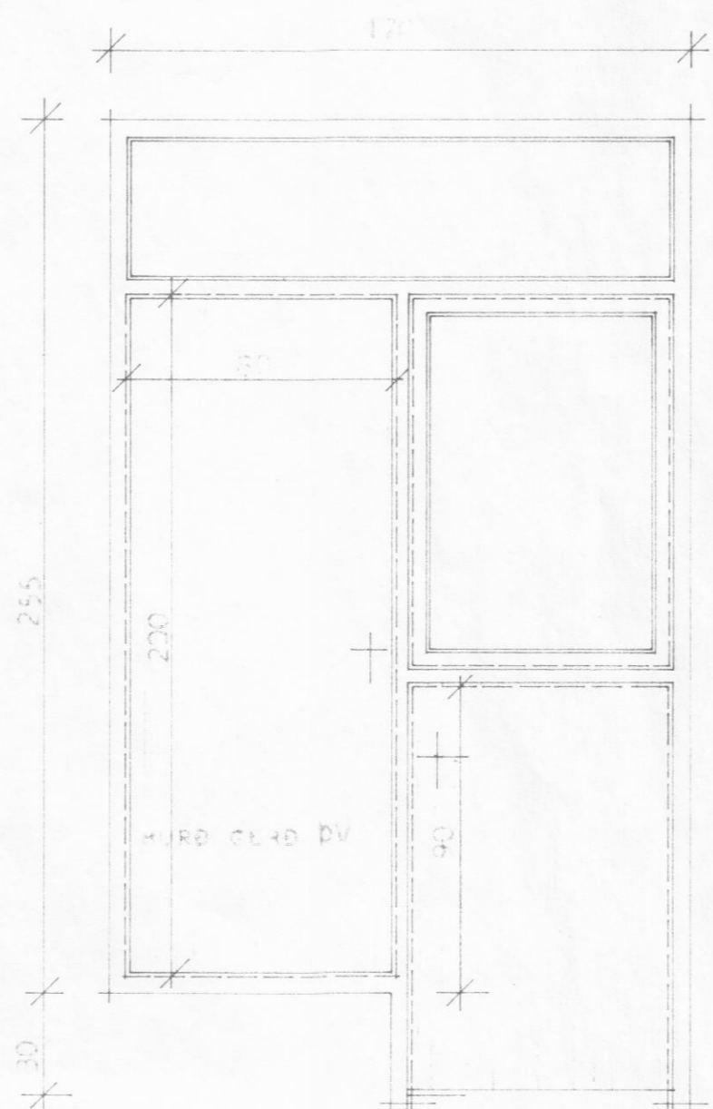
1 STK. HURD-GJAFURD.
