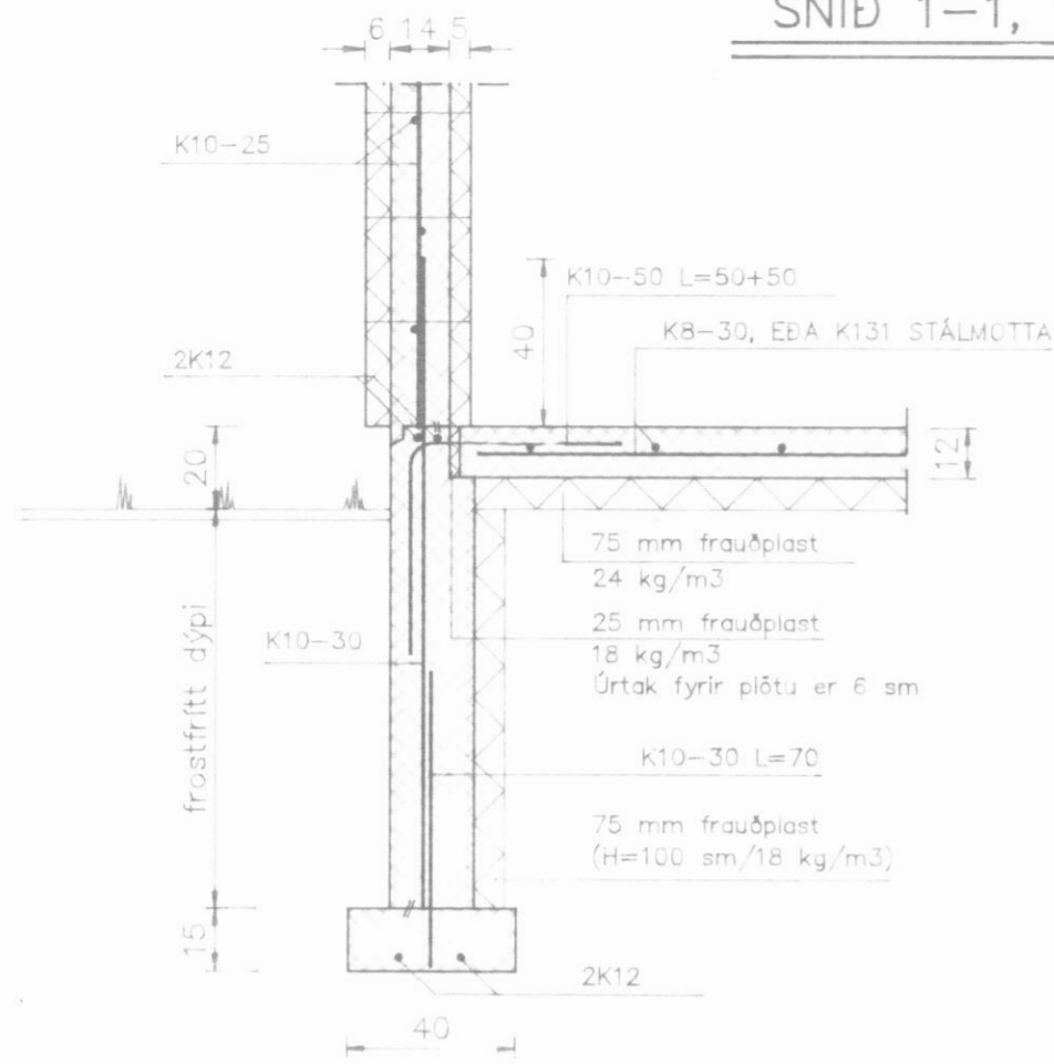
SNID 1-1, 1:20
