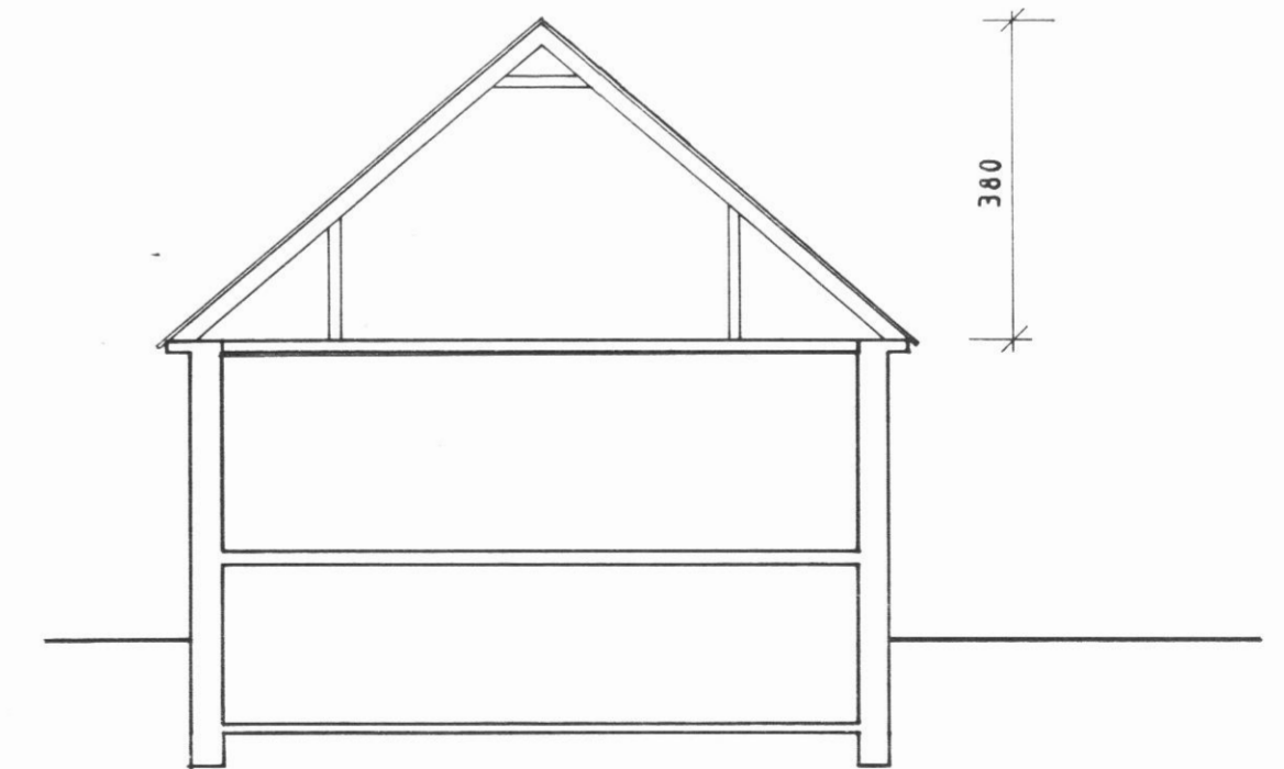
SNID BB
